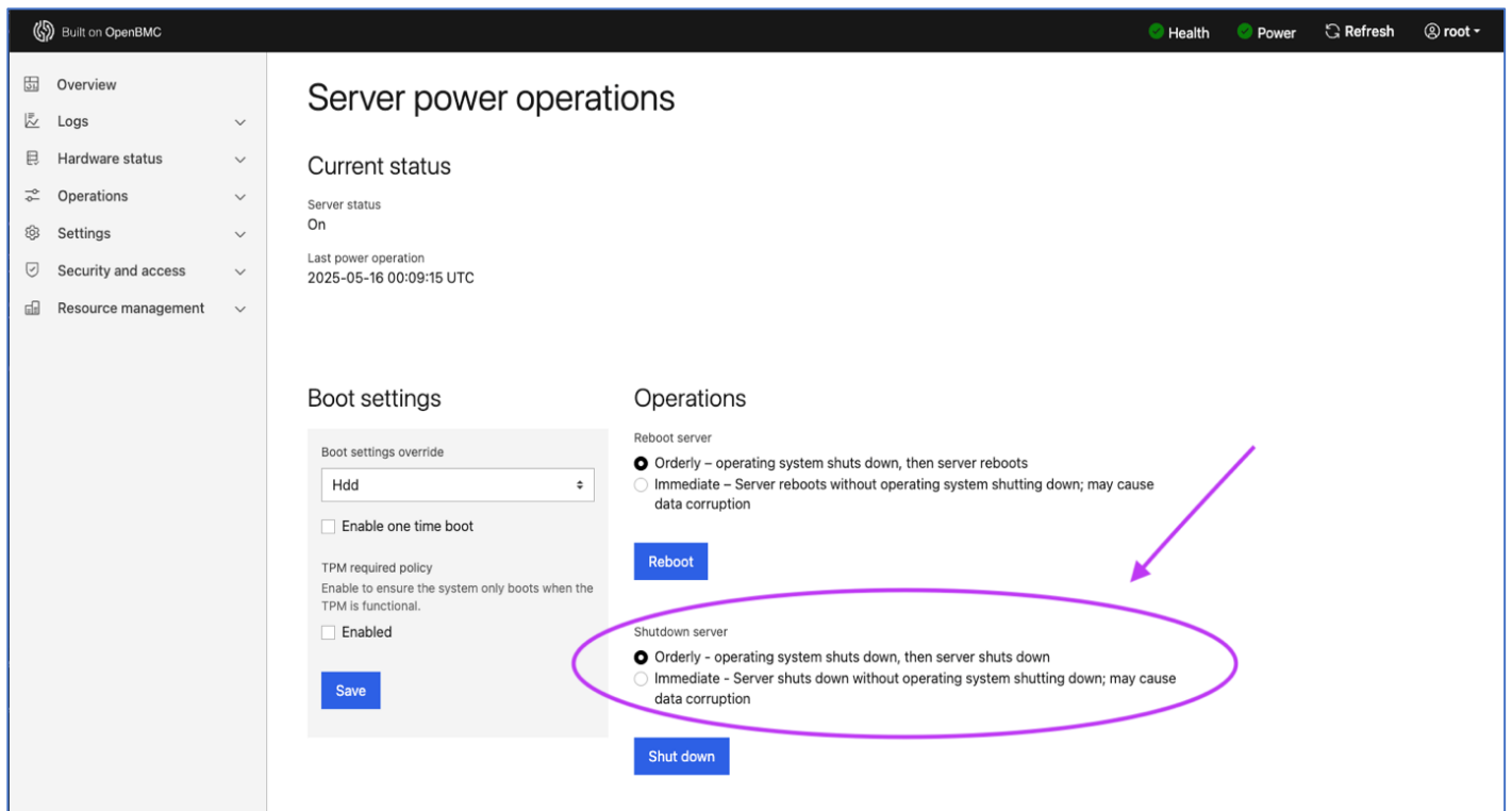
Figure 18 Screenshot of Orderly Shutdown Option in BMC
