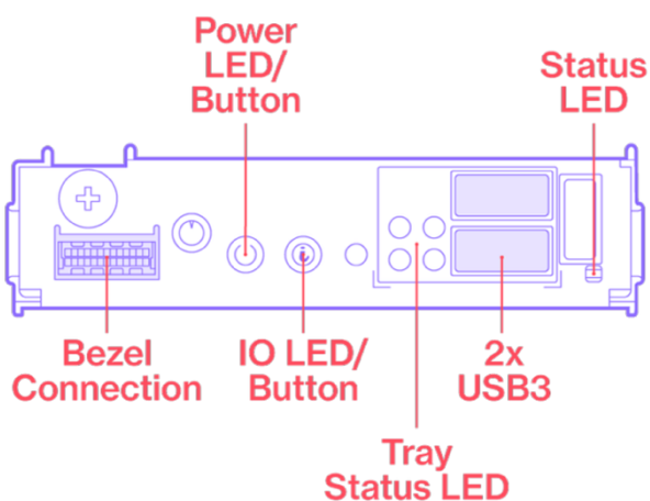
Figure 8 Front Control Panel
