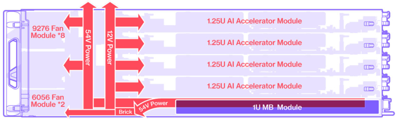
Figure 11 Power Block Diagram
