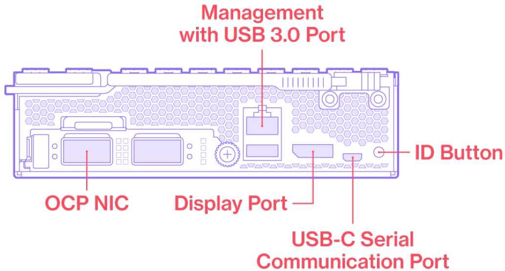
Figure 10 Rear I/O View
