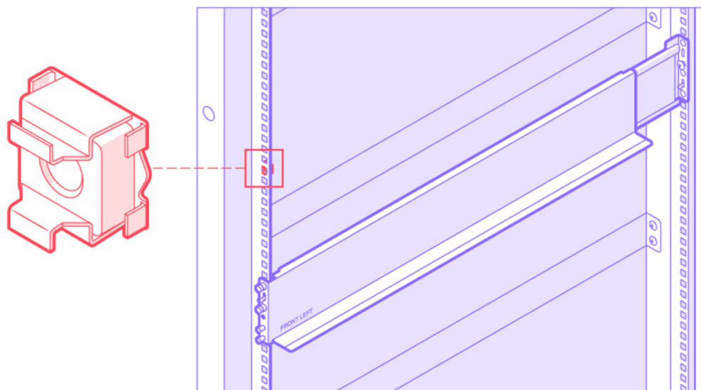
Figure 13 Rack Nut Placement
