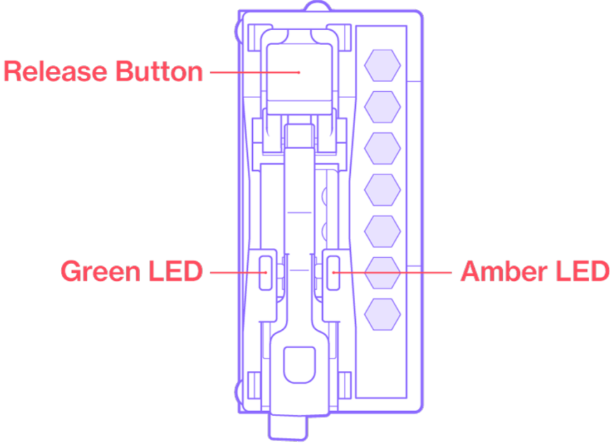
Figure 7 E1.S Overview
