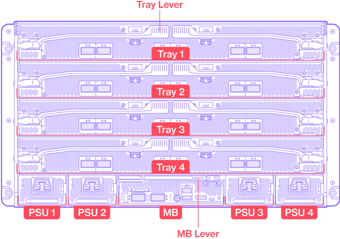
Figure 9 System Rear View
